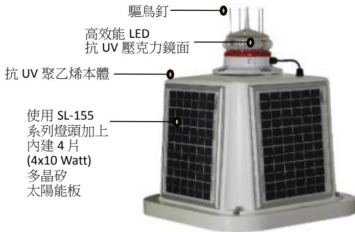
SL-C500 (5-12NM)
